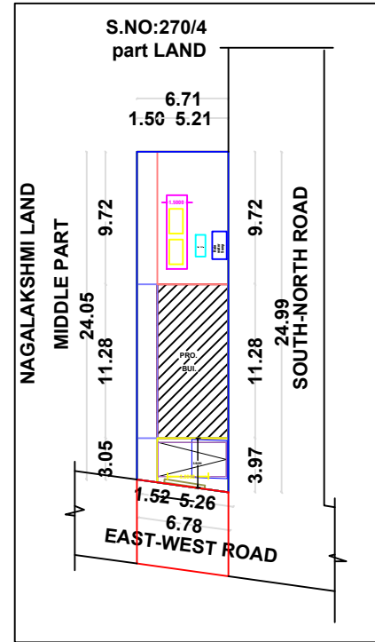
SITE PLAN & KEY PLAN
