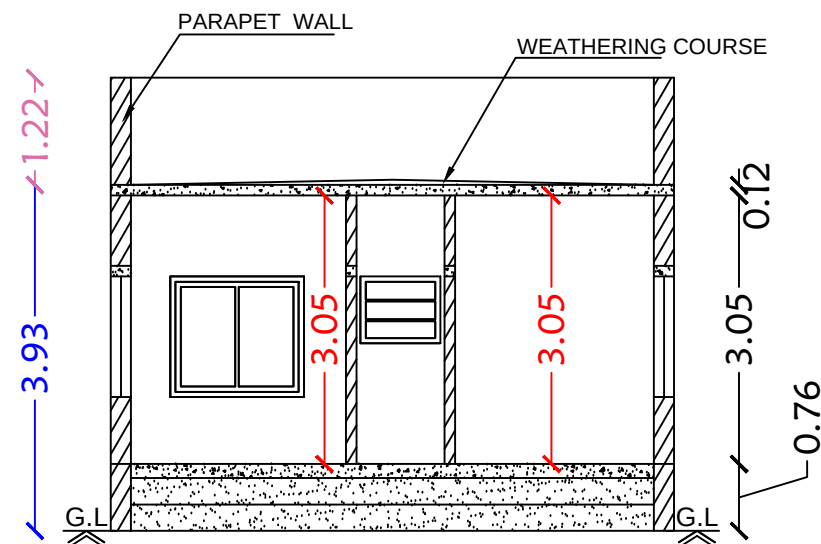
Section on-"AA"
