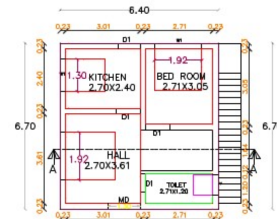
GROUND FLOOR PLAN PROPOSED
