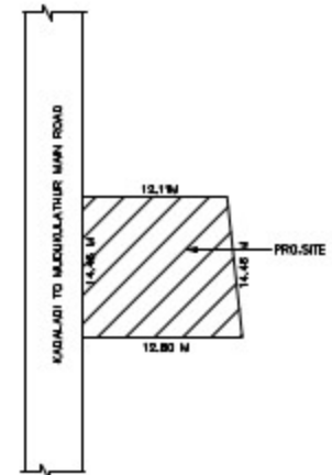
TOPO PLAN
