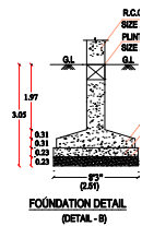
FOUNDATION DETAIL (DETAIL - B)
