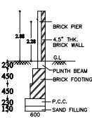
COMPOUND WALL
