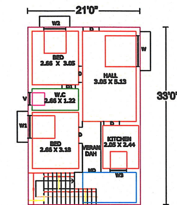
EXIST.GROUND FLOOR PLAN
