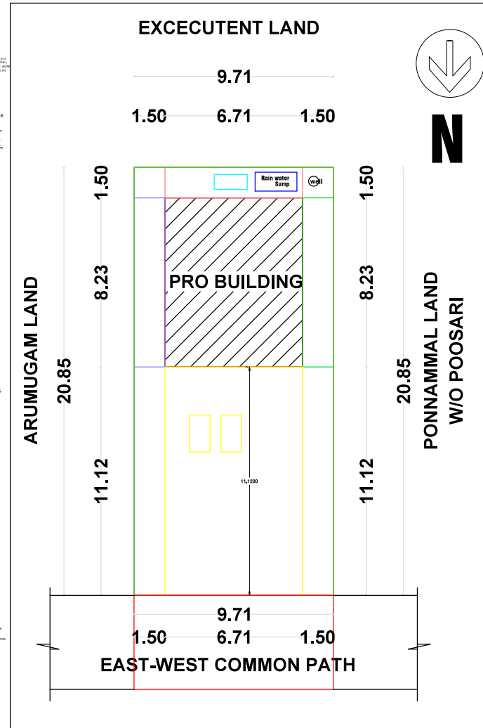
SITE PLAN & LOCATION
