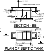
SECTION - BB PLAN OF SEPTIC TANK
