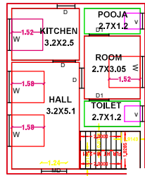
GROUND FLOOR P
