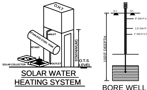
BORE WELL
