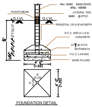
FOUNDATION DETAIL
