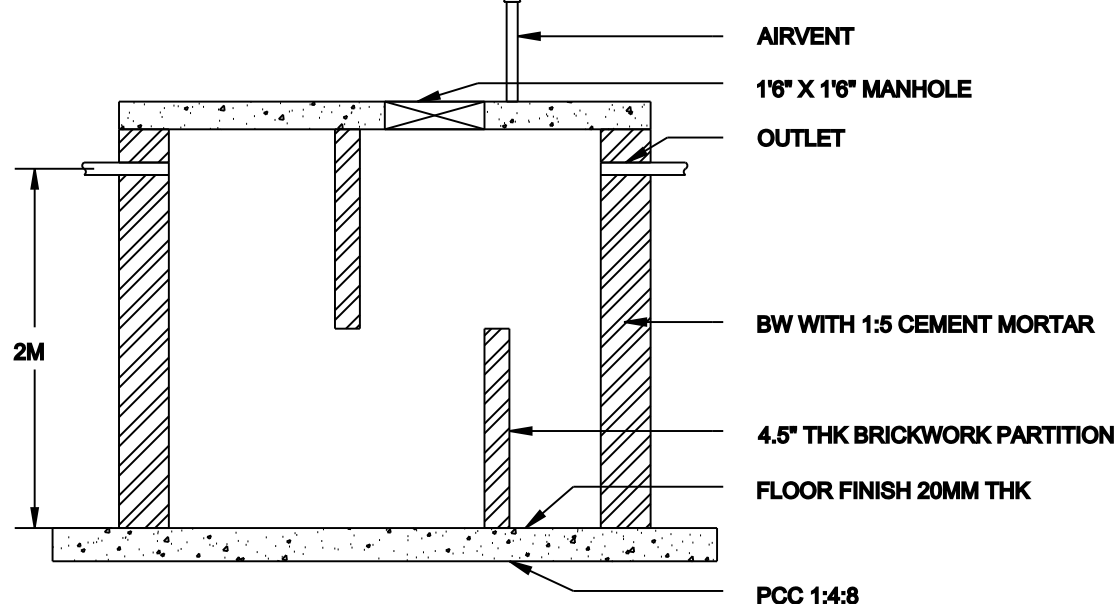
CROSS SECTION OF SEPTIC TANK
