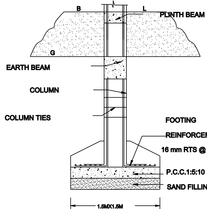
FOUNDATION DETAIL
