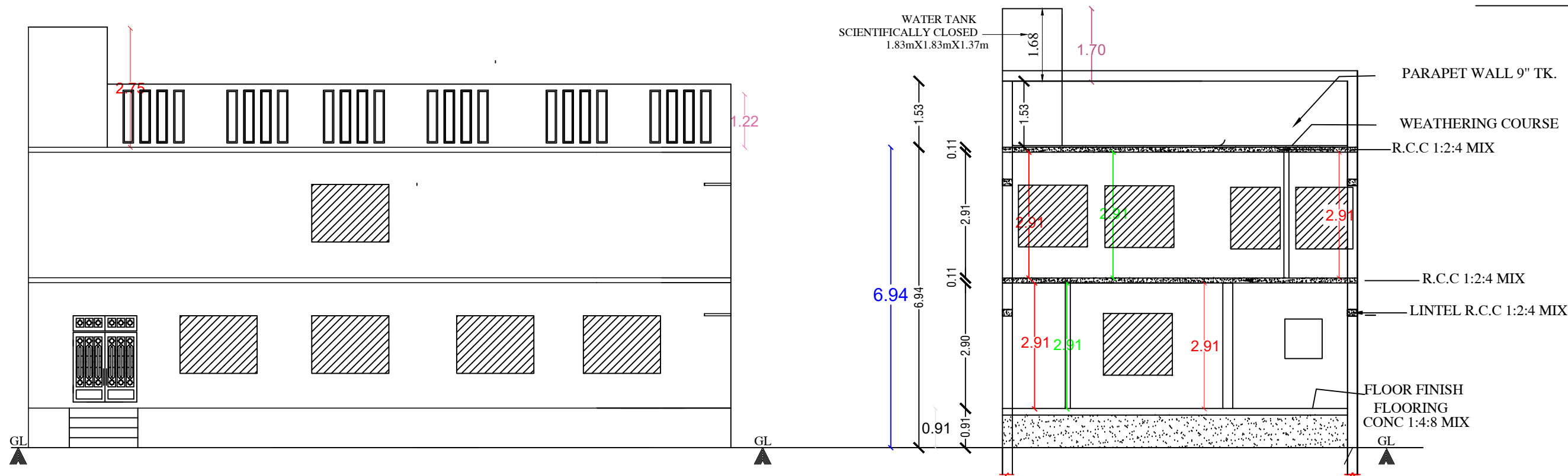
FRONT ELEVATION
