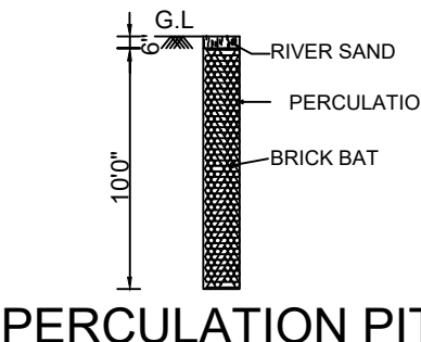
PERCOLATION PIT
