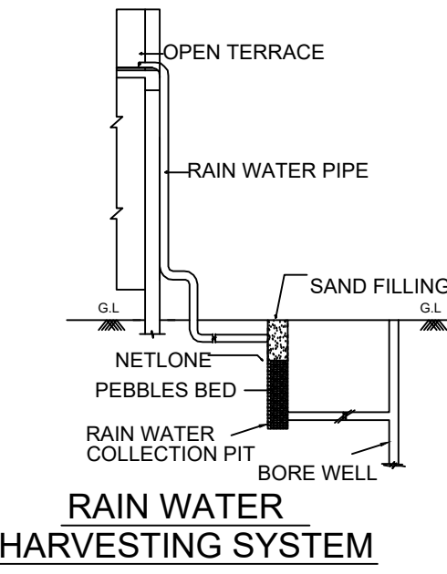
BORE WELL
