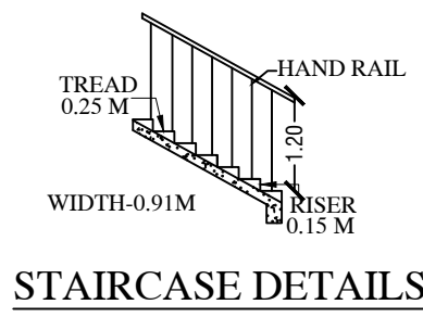
STAIRCASE DETAILS
