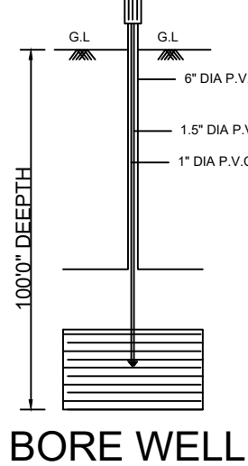
BORE WELL
