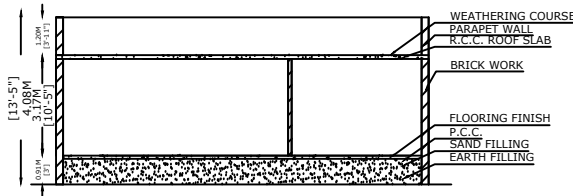
SECTION AN AA
