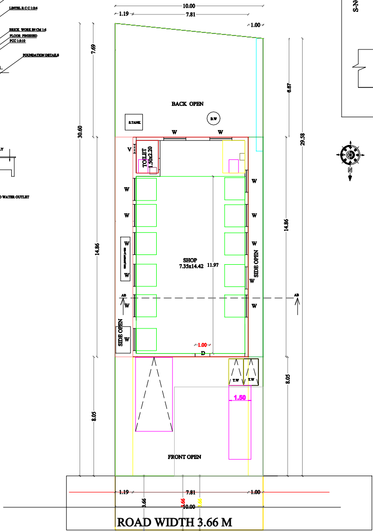
SITE PLAN
