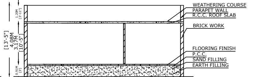
SECTION AN AA
