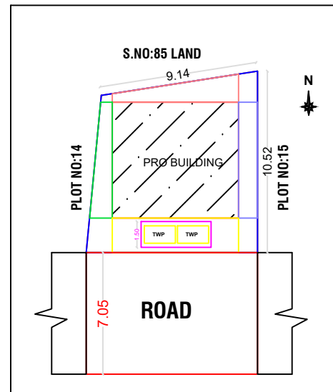
SITE PLAN
