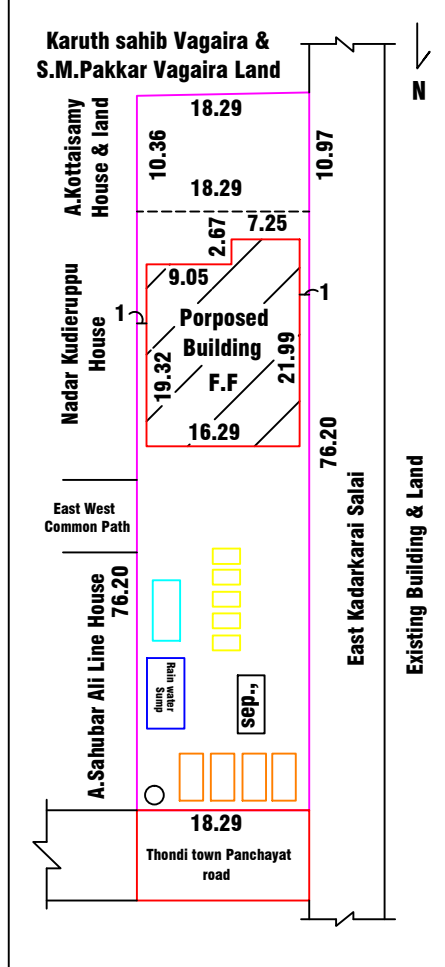
SITE PLAN CUM KEYPLAN
