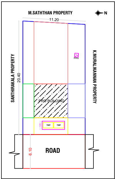
SITE PLAN
