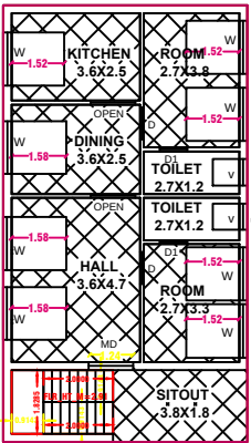
EXISTING GROUND FLOOR PLAN
