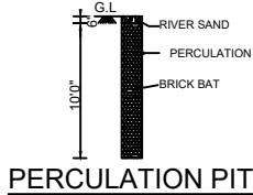
PERCOLATION PIT
