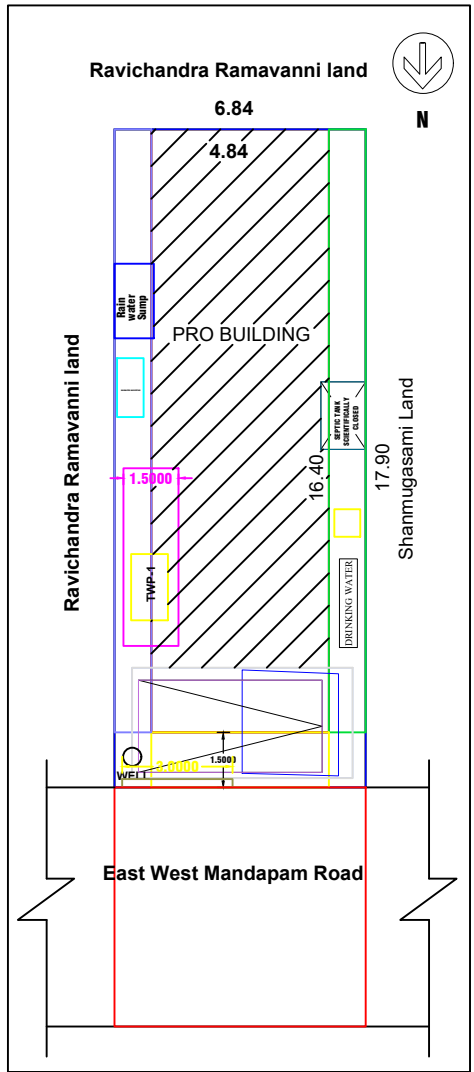
SITE PLAN & KEY PLAN
