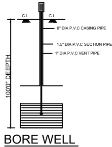
BORE WELL
