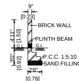
SECTION - CC
