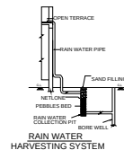
RAIN WATER HARVESTING SYSTEM
