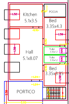
SITE PLAN CUM GROUND FLOOR PLAN
