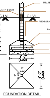
FOUNDATION DETAIL
