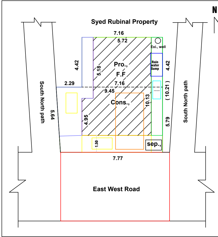
SITE PLAN & KEY PLAN (1:100)
