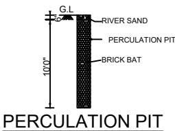
PERCOLATION PIT
