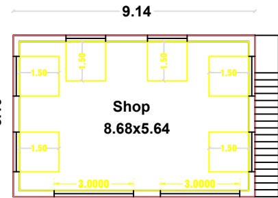
PRO. GROUND FLOOR PLAN
