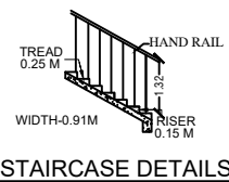
STAIRCASE DETAILS
