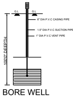
BORE WELL
