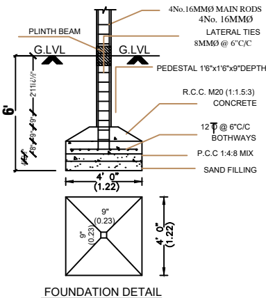
FOUNDATION DETAIL
