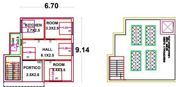
R PLAN
