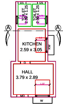
PROPOSED GROUND FLOOR
