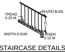
STAIRCASE DETAILS
