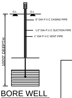
BORE WELL
