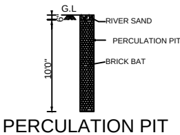
PERCOLATION PIT
