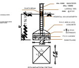
COMPOUND WALL
