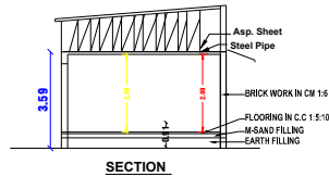
SECTION
