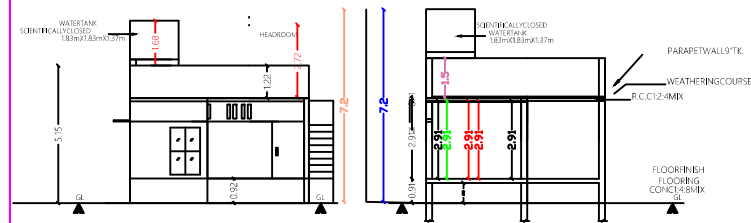
FRONT ELEVATION
