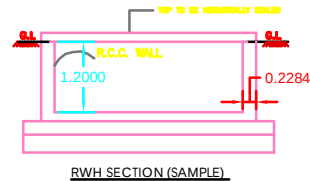
RWH_CAPACITY_L=2000LTRS
