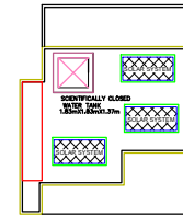
TERRACE FLOOR PLAN
