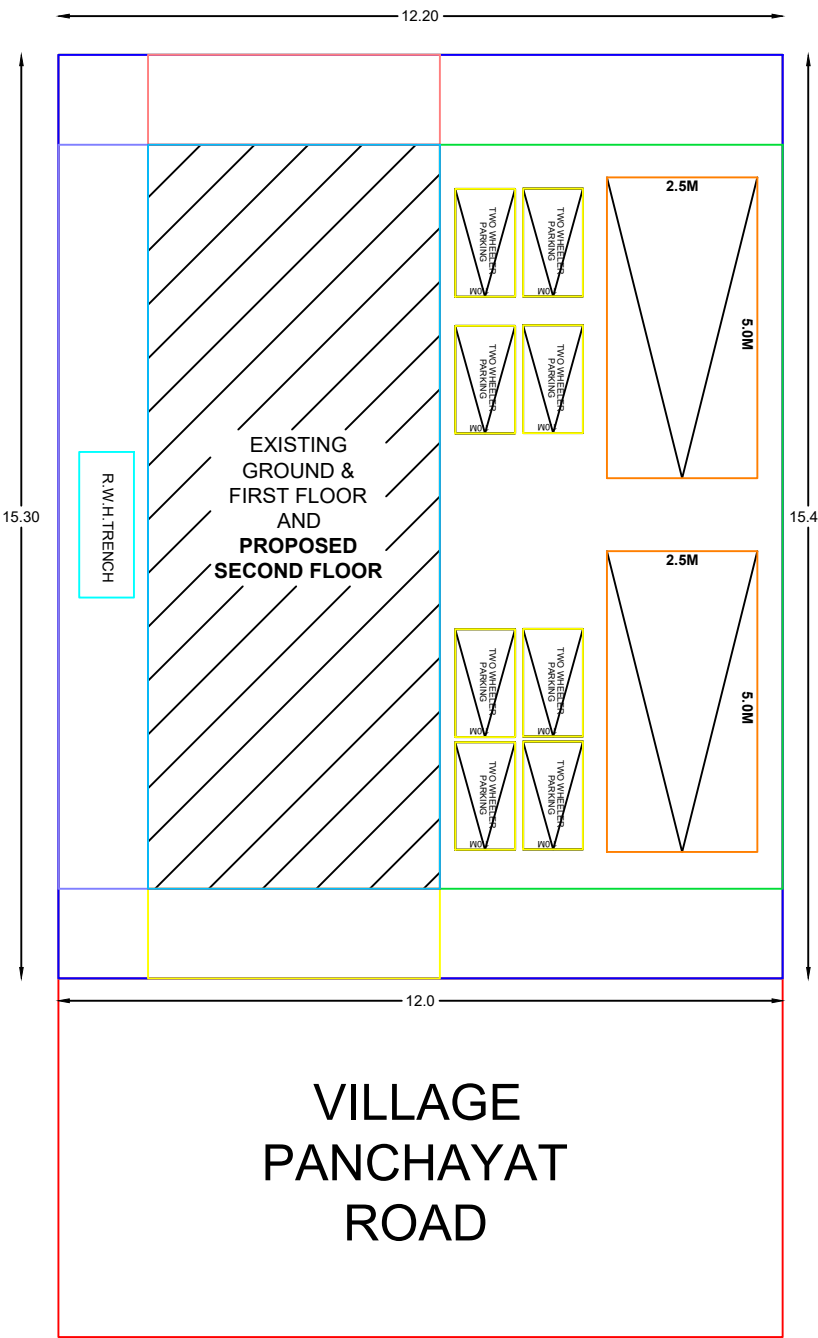
SITE PLAN
