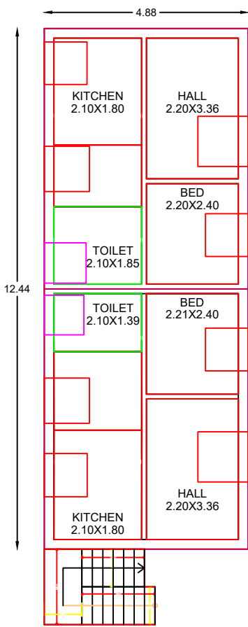
EXISTING FIRST FLOOR PLAN
