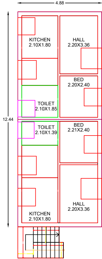
EXISTING GROUND FLOOR PLAN
