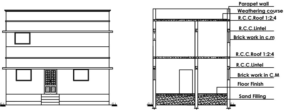
ELEVATION SECTION ON XX
