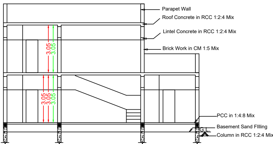
Section RR
