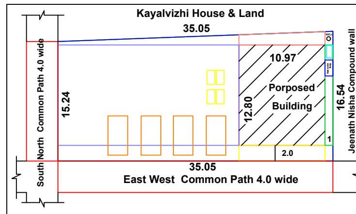
SITE PLAN CUM KEYPLAN
