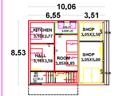
GROUND FLOOR PLAN COMMERCIAL & RESIDENTIAL
