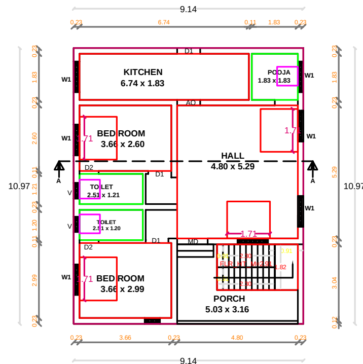
GROUND FLOOR PLAN PROPOSED
