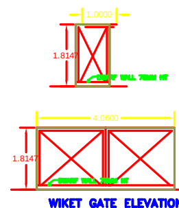
WIKET GATE ELEVATION
