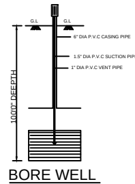
BORE WELL
