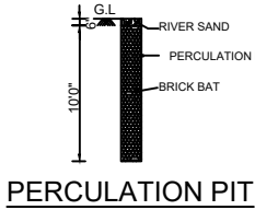
PERCOLATION PIT
