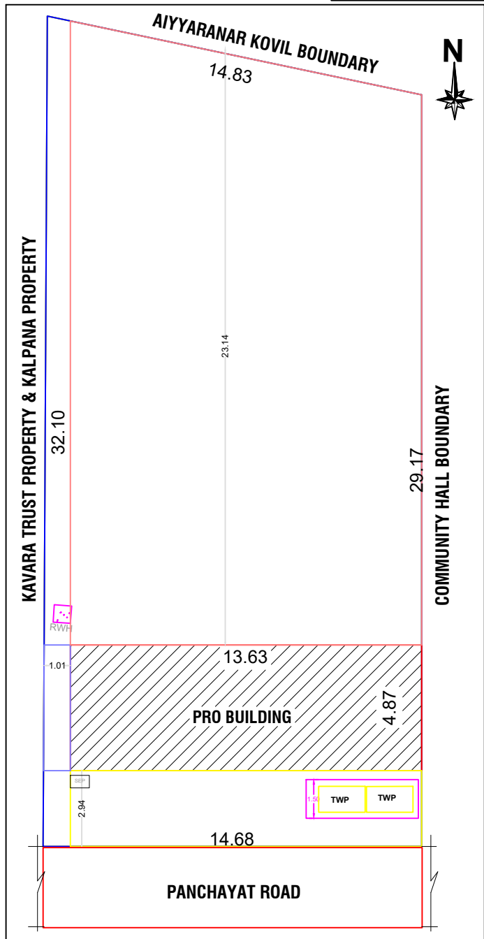
SITE PLAN
