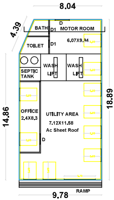
PRO. GROUND FLOOR PLAN
