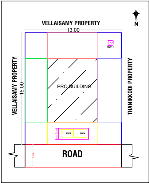
SITE PLAN
