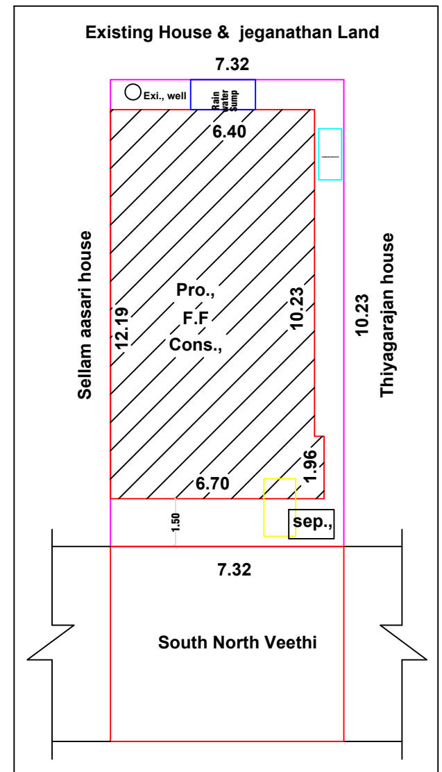
SITE PLAN & KEY PLAN (1:100)
