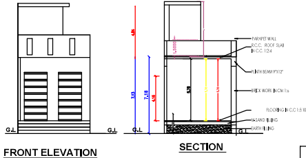
FRONT ELEVATION
