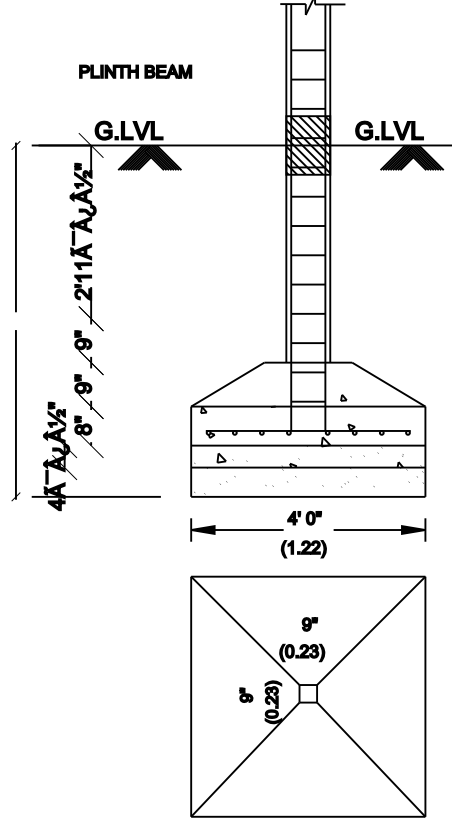
FOUNDATION DETAIL
