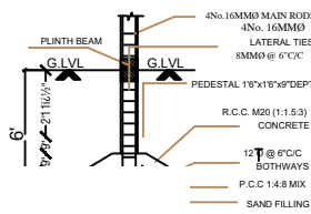
Detail Scale
