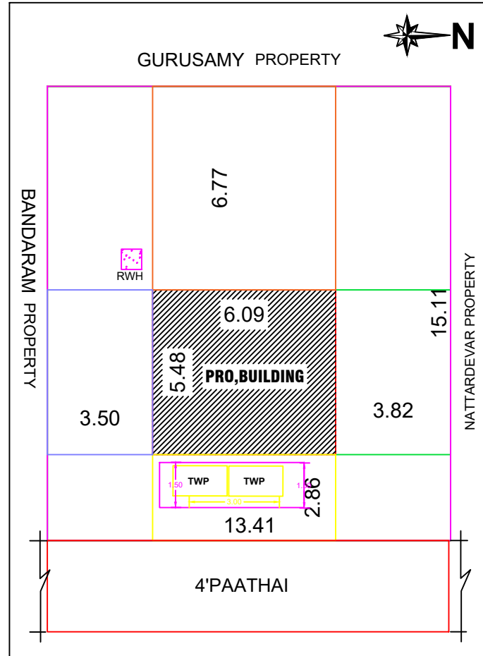
SITE PLAN
