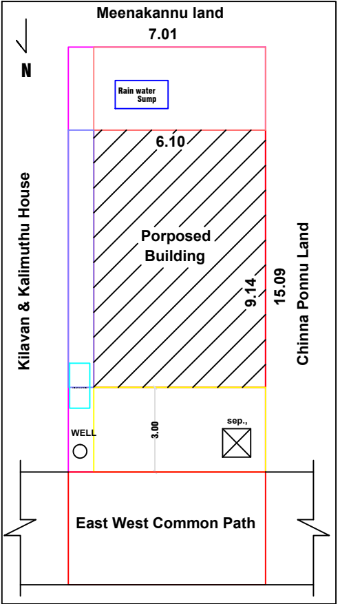
SITE PLAN CUM KEYPLAN
