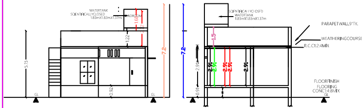
FRONT ELEVATION
