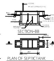
ELEVATION SECTION-BB
