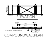
COMPOUND WALL PLAN
