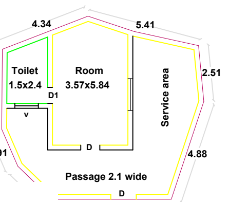
IO. GROUND FLOOR PLAN
