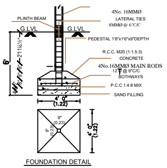
FOUNDATION DETAIL
