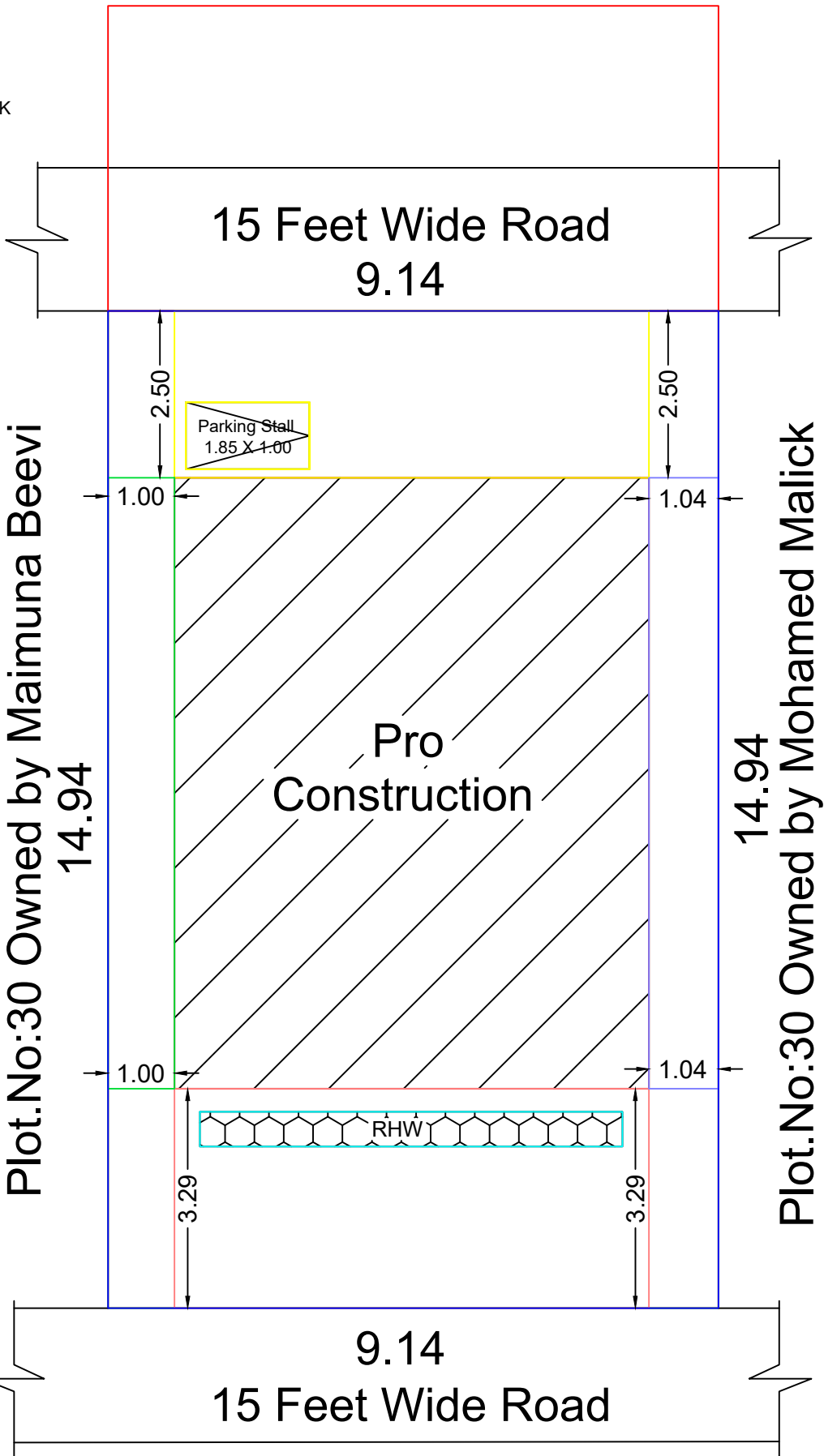
Site Plan
