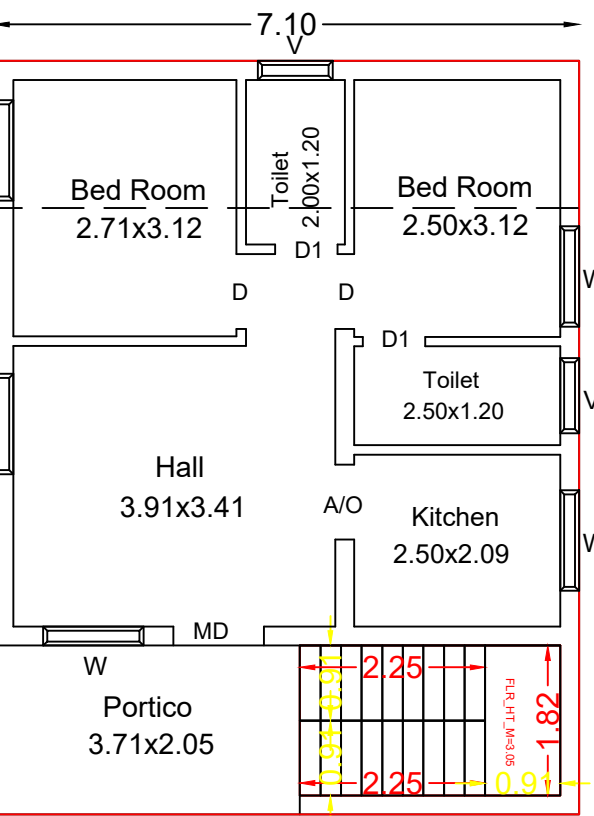
Ex.Ground Floor Plan
