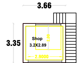
PRO. GROUND FLOOR PLAN
