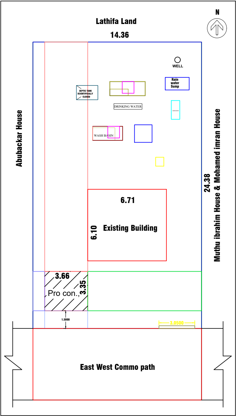
SITE PLAN & KEY PLAN
