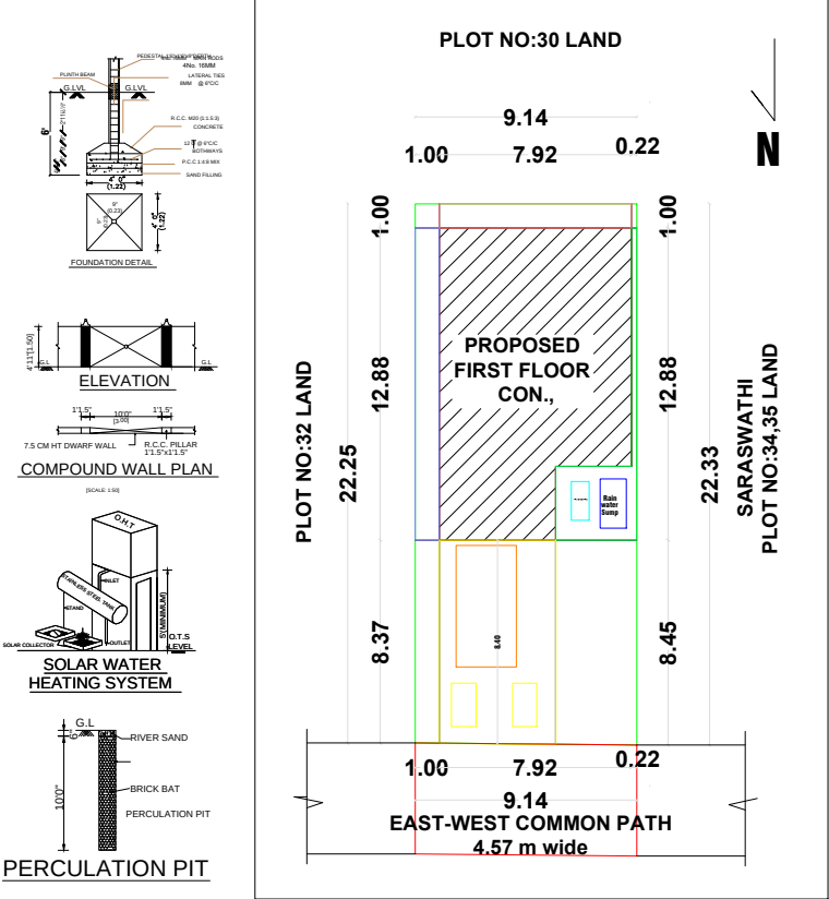
SITE PLAN & KEY PLAN (1:100)
