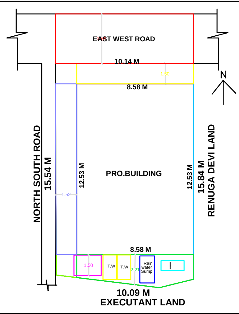
SITE PLAN PROPOSED
