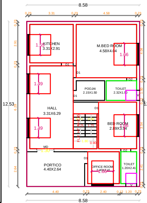
GROUND FLOOR PLAN PROPOSED
