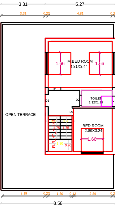
FIRST FLOOR PLAN PROPOSED
